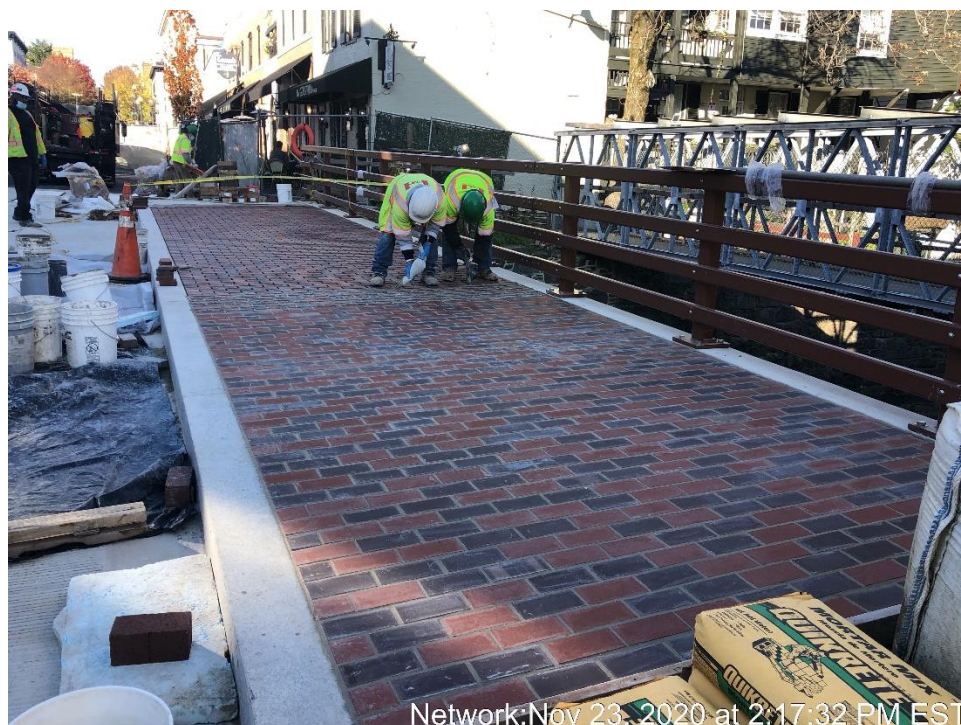
Construction of Brick Sidewalk – East Side of the Bridge
